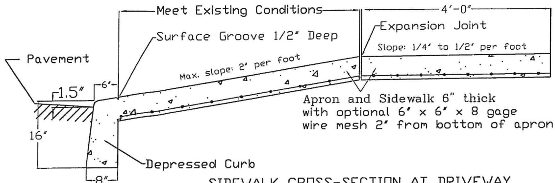
SIDEWALK CROSS-SECTION AT DRIVEWAY
